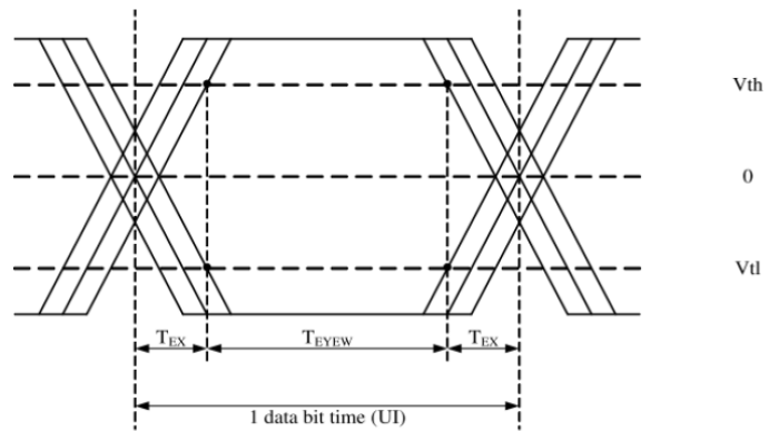
LVDS input eye diagram
